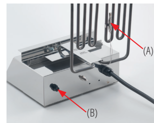
(A) Bulbo termostato (B) Pulsante di ripristino cut-off (A) Thermostat bulb (B) Cut-off reset button
