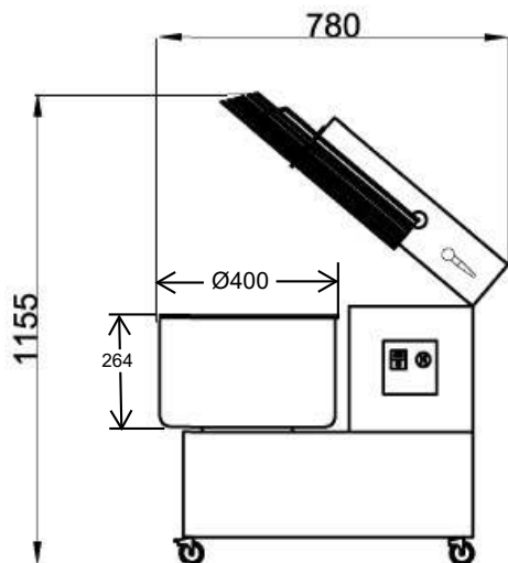
Rear side
