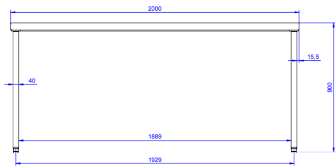
Front
