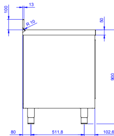
Side
