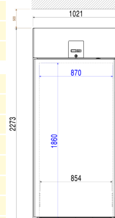
Front
