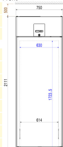
Front
