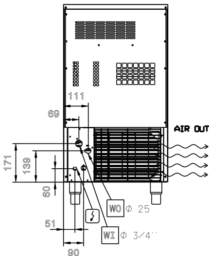
Rear side
