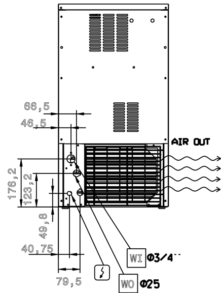
Rear side
