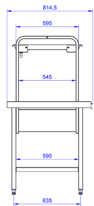
Side
