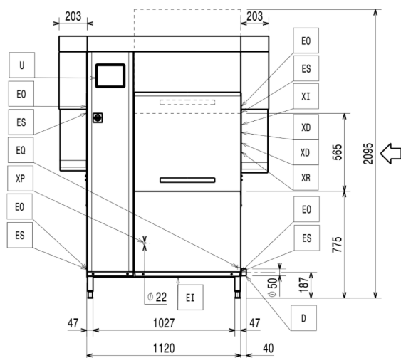
Front
