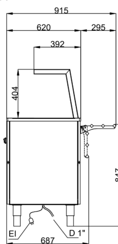
Side
