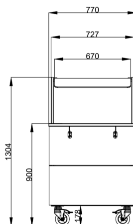
Front
