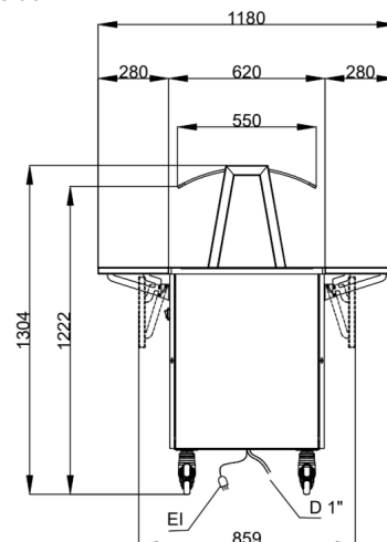
Side
