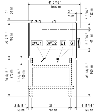
Side
