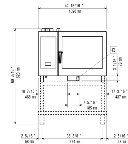
Front
