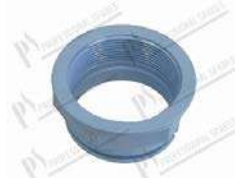
Nut for wash arm support Ø 53.2x74x35 mm; CH 65 mm; left wash system
